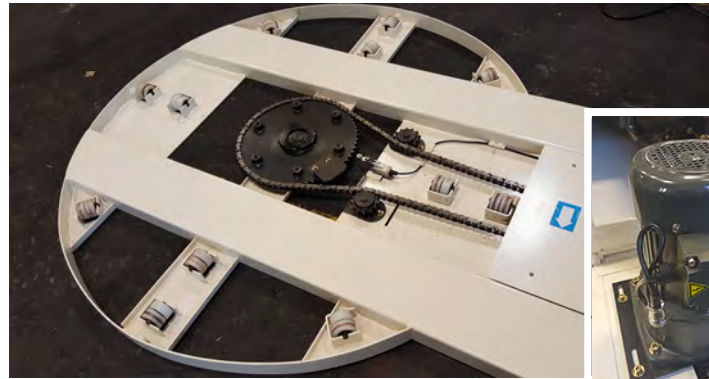
(24) Heavy-Duty Sealed Bearing Nylon Rollers
